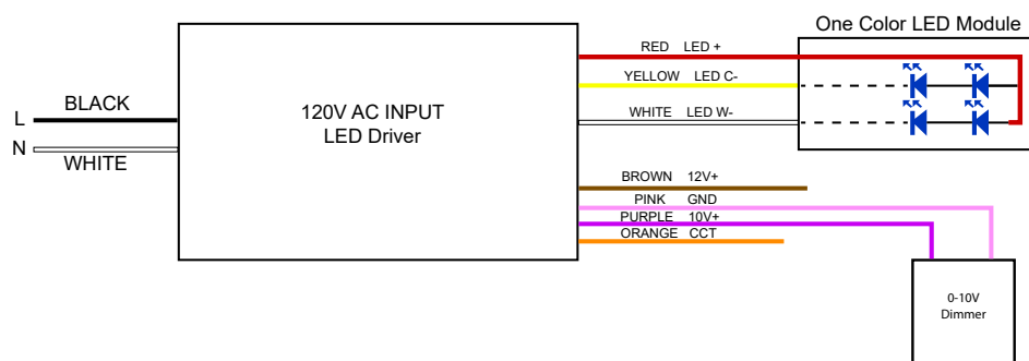
Single Channel LED with 0-10V Dimming
