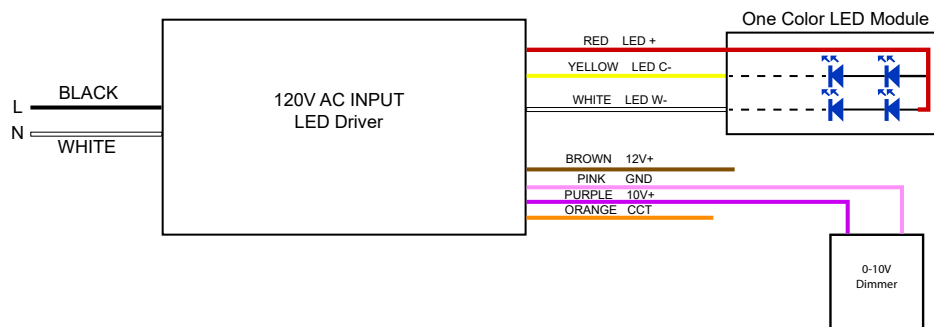
Single Channel LED with 0-10V Dimming
