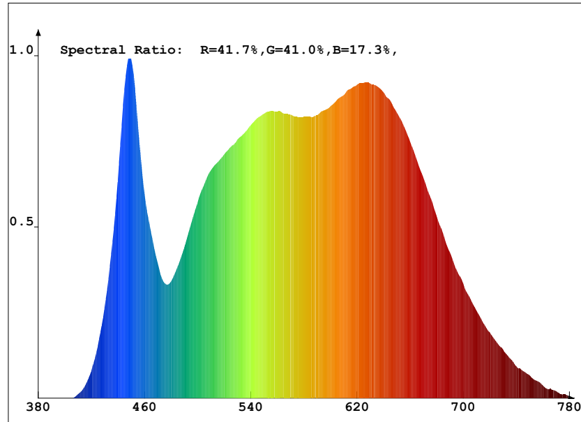
Diagram shown is based on the test report for 80 CRI 4000K model.
